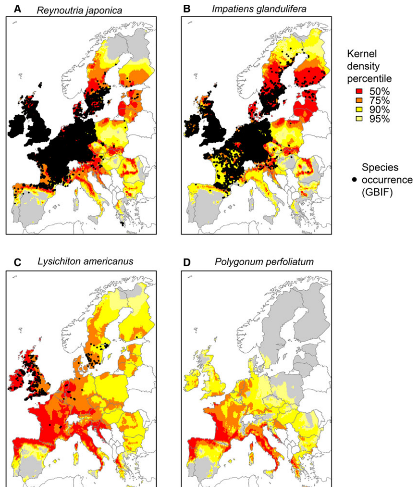
Fig. 3 Crude estimates of the climatically suitable regions of the EU for (A) Reynoutria japonica , (B) Impatiens glandulifera , (C) Lysichiton americanus and (D) Polygonum perfoliatum . Global occurrence locations were obtained from the Global Biodiversity Information Facility (GBIF). The authors acknowledge that GBIF occurrence data are not exhaustive, especially for R. japonica and I. glandulifera . The global climate was summarized as two principal components analysis (PCA) axes on the 19 WorldClim layers (Hijmans et al. , 2005). Species occurrences were plotted in this climate space and a bivariate normal kernel density model (Calenge, 2006) was used to estimate 'climate envelopes' at different percentiles. These envelopes were then projected onto geographical space in the EU. Shading indicates these percentiles, with smaller numbers indicating higher density of occurrences. Species with regions inside the smaller kernel density percentiles without species occurrences (black points) may have a significant area for further spread and establishment in the EU.
